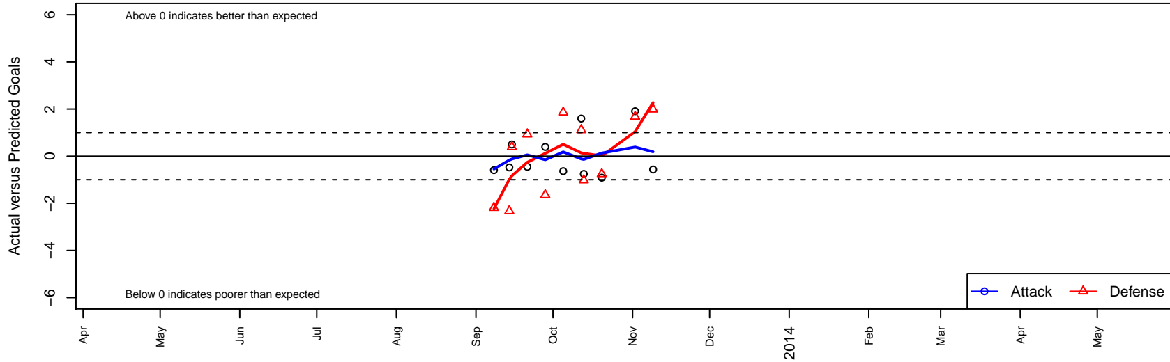
IE Surf Peters B98 Dots are actual minus expected GF (blue circles) and GA (red triangles). Blue line is smoothed change in attack strength. Red is smoothed change in defense strength.
